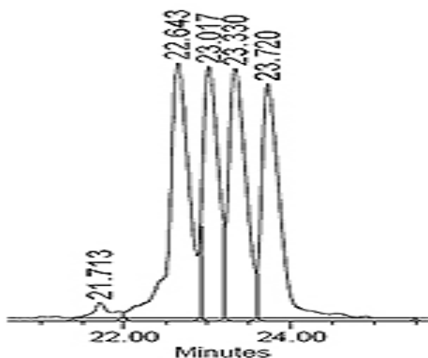
HPLC Separation Profile of a Mixture of Oligos with Wobble Based Pair
